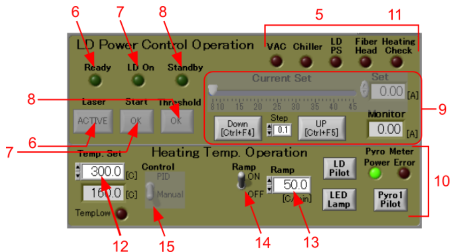
Figure 11: Substrate heating operation on PC control software.
