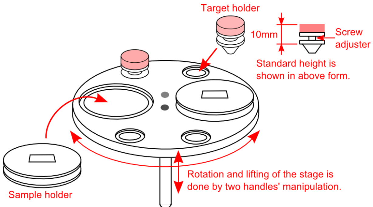
Figure 3:Substrate holder/target holder setting in load-lock chamber.
