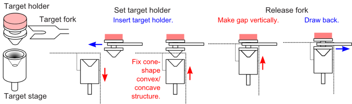
Figure 7: Target holder transfer to the target stage in the main chamber.
