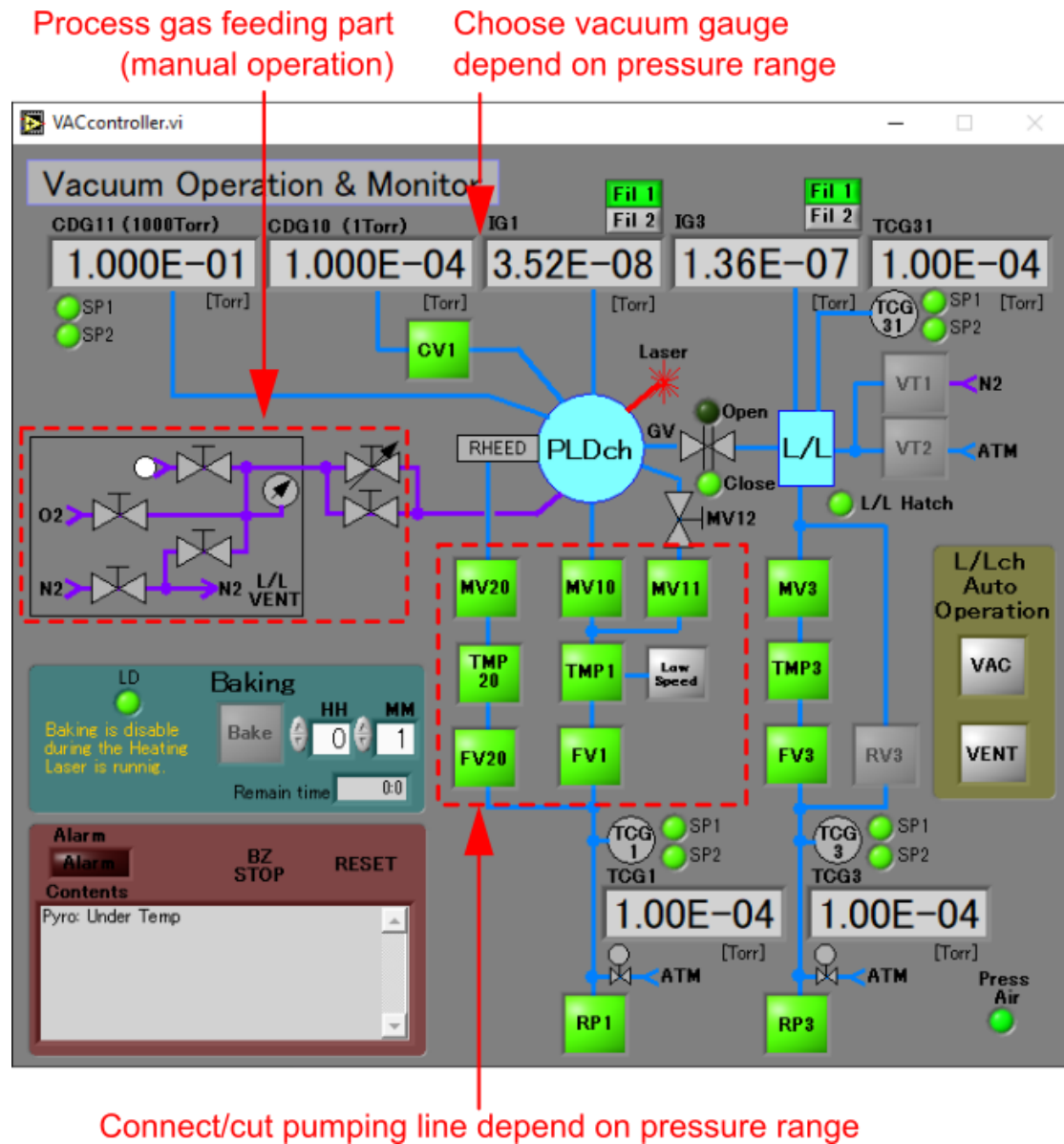
Figure 9: Gas feeding part in control software.
