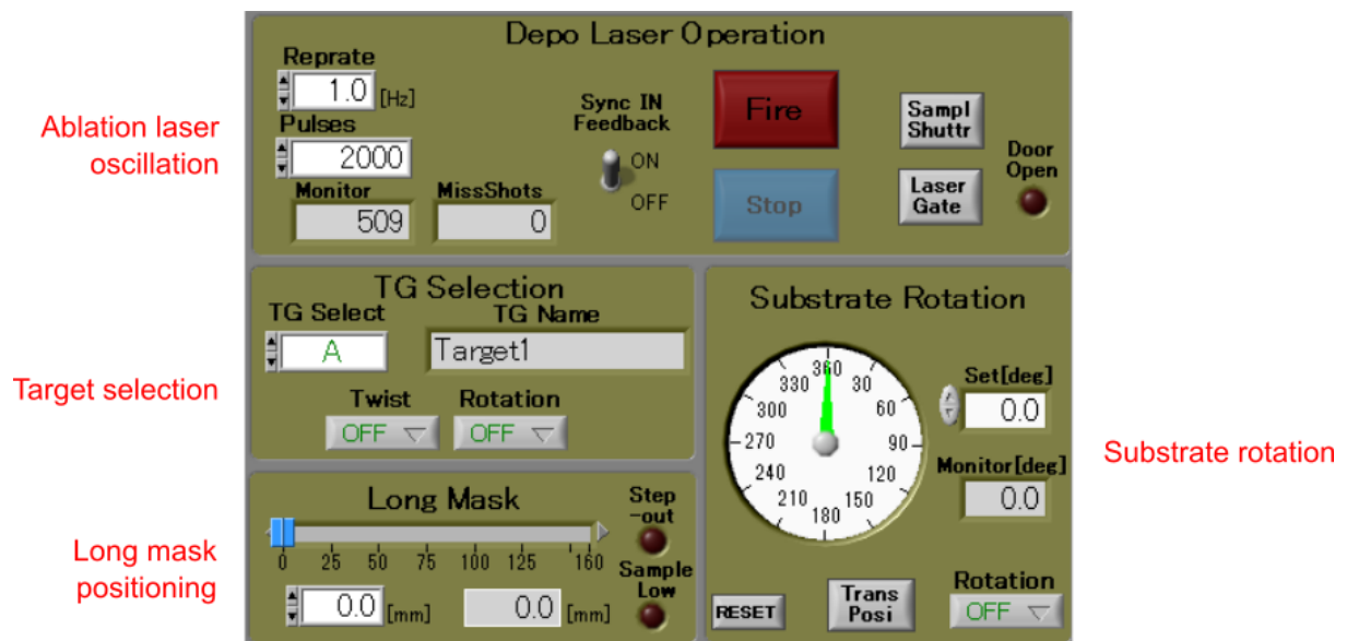
Figure 12: Other control objects on PC control software.
