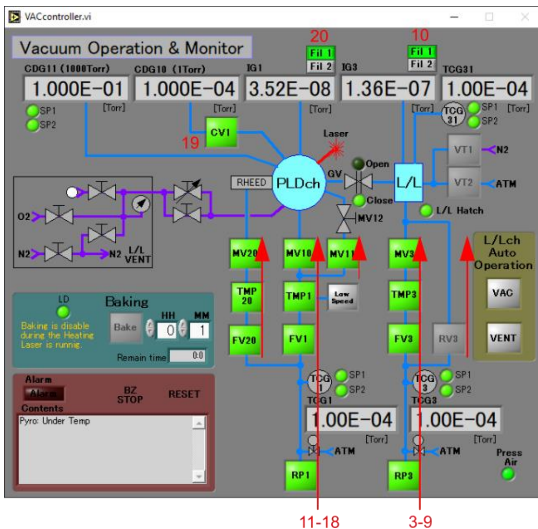
Figure 1: Vacuum pumping operation in PC control software.
